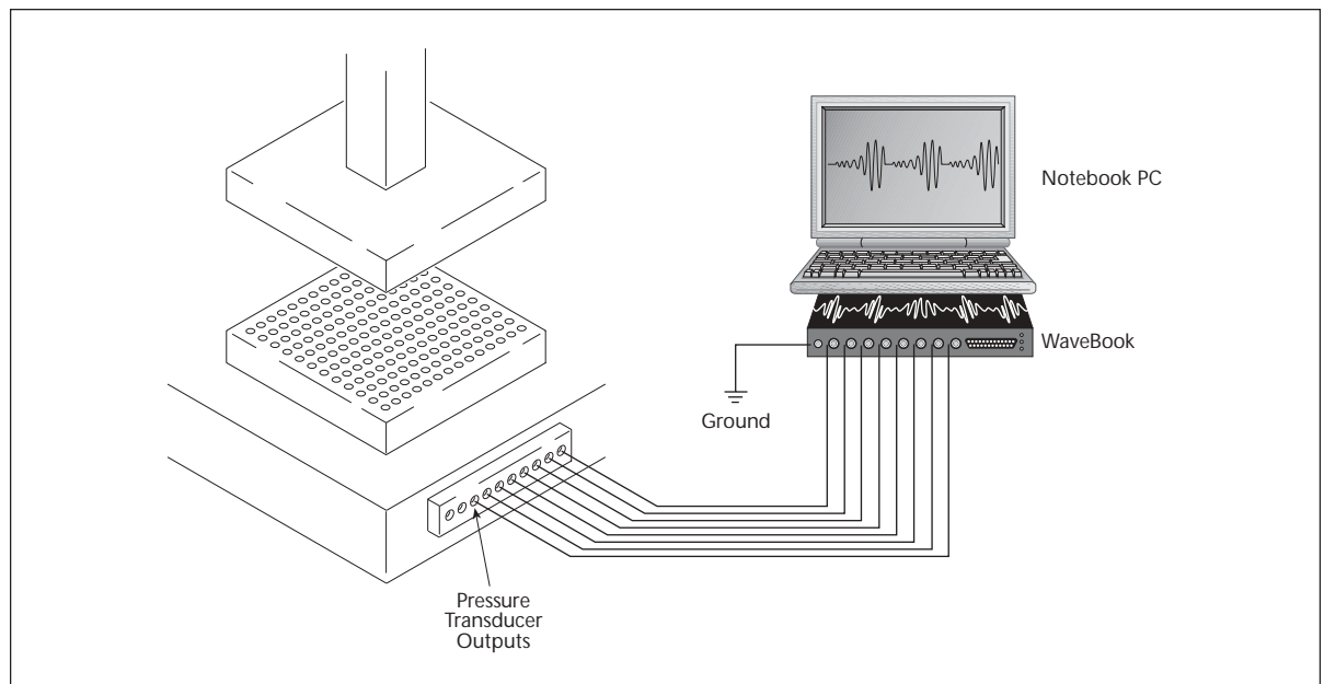
Process-control set-up
