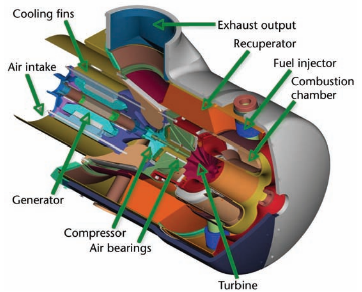
Microturbine Diagram
